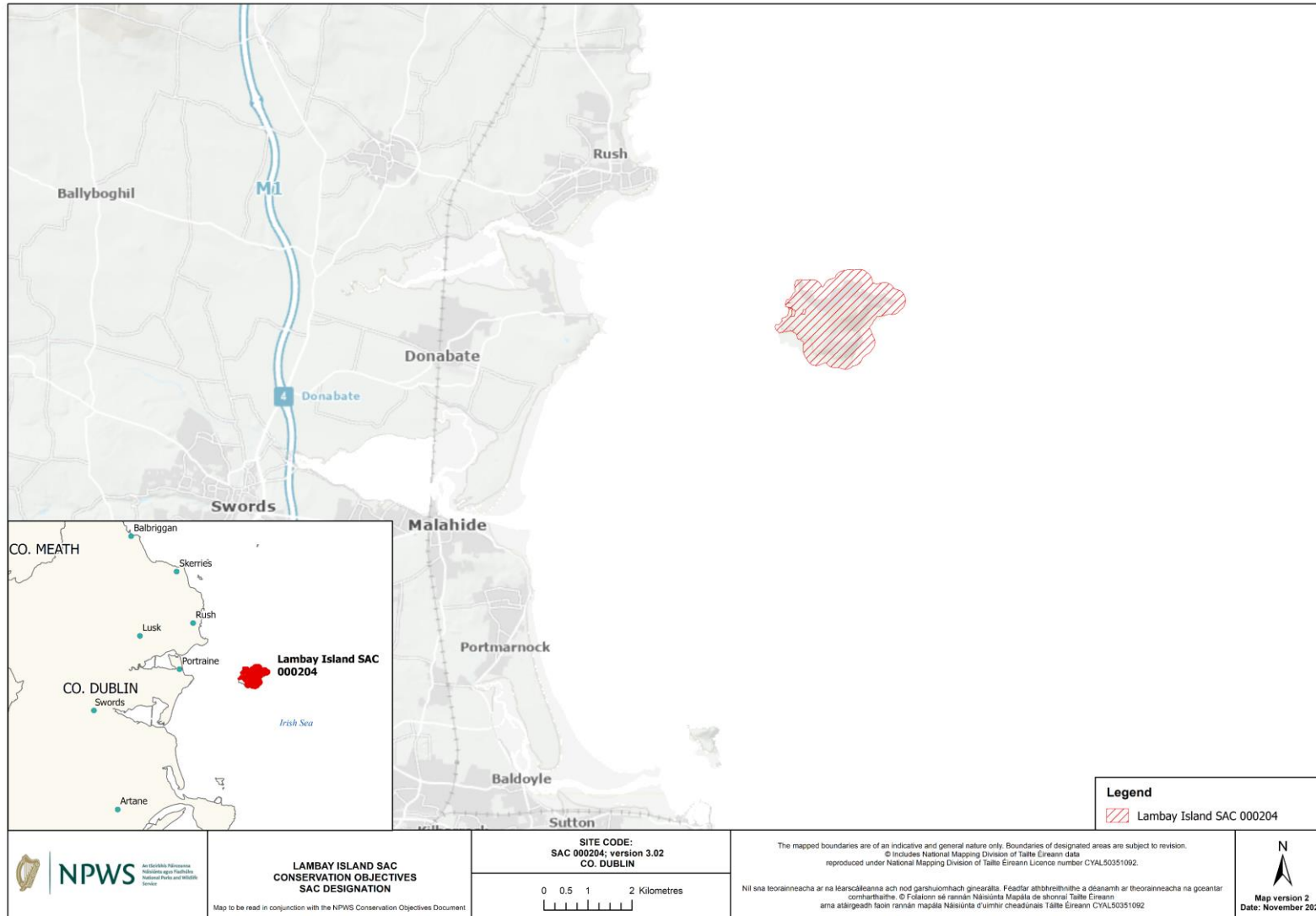
Figure 1. Suitable habitat for Phocoena phocoena within Lambay Island SAC
